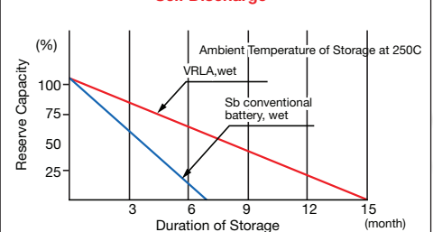
Self Discharge
